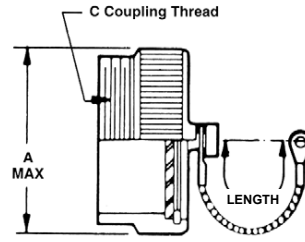
TF261 PLUG CAP
